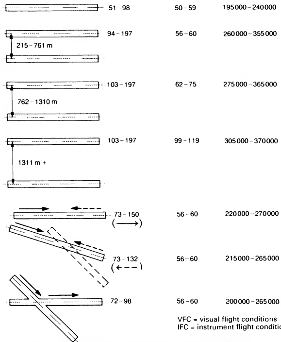
1 Capacity of different take-off/landing runway systems
